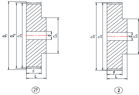
T2.5-16 Pitch = 2.5mm For belt width 6mm
